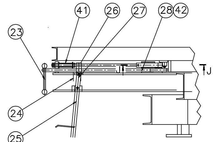
SECTION E-E
